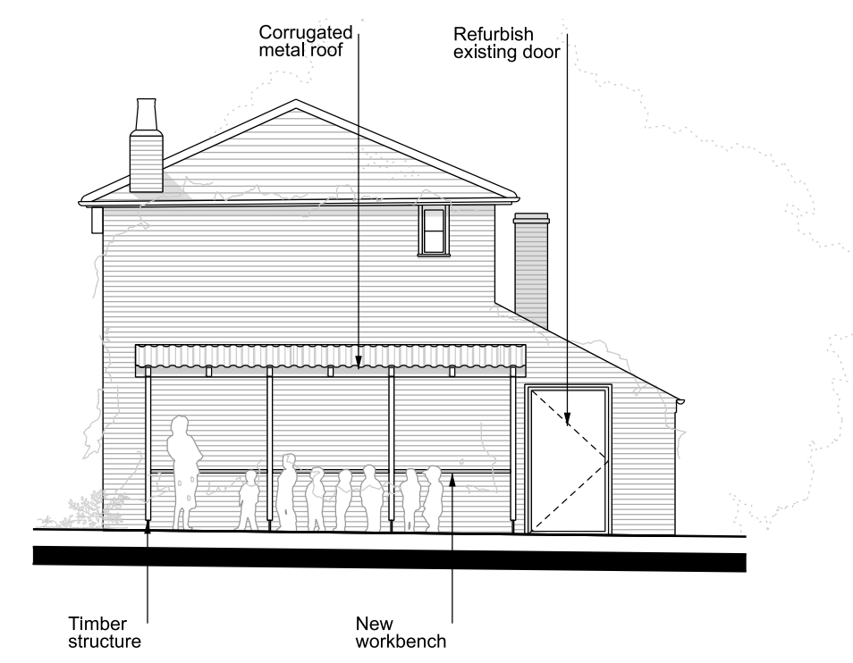
02 0202 Proposed Drawings Stables 1:100@A3 South East Elevation
