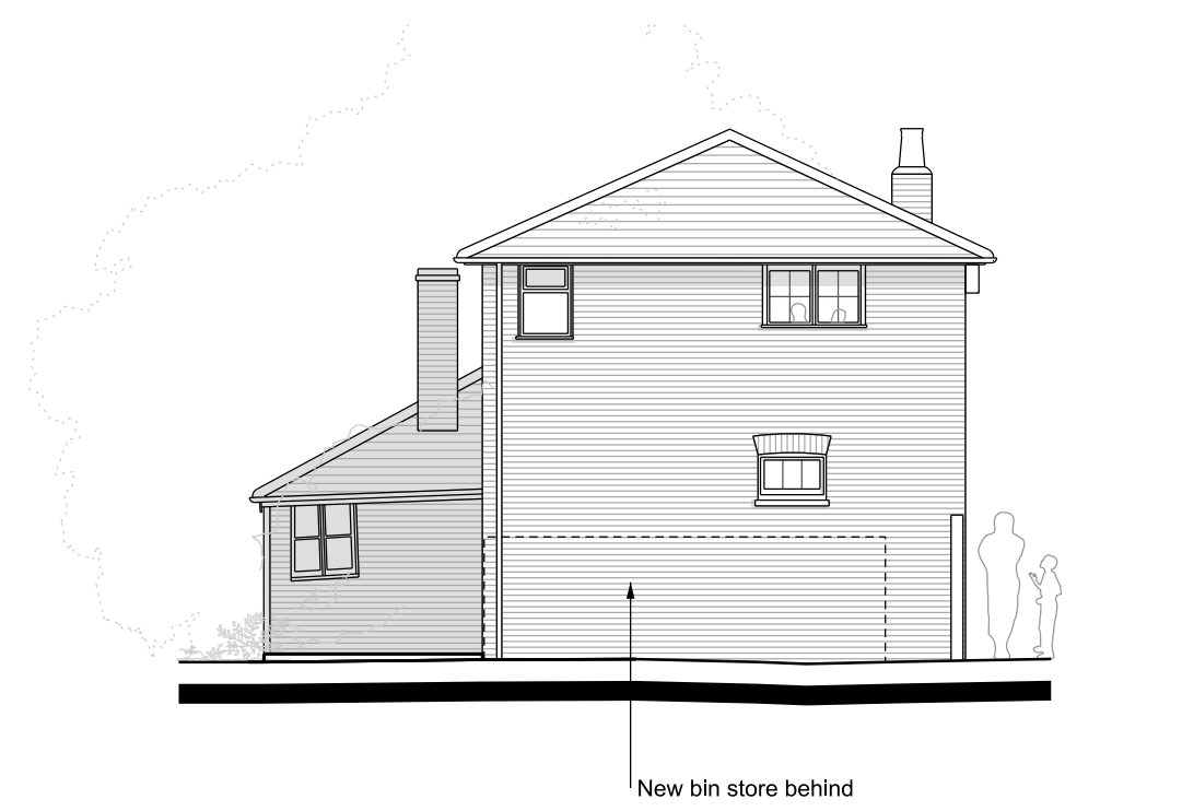
04 0202 Proposed Drawings Stables 1:100@A3 North West Elevation
