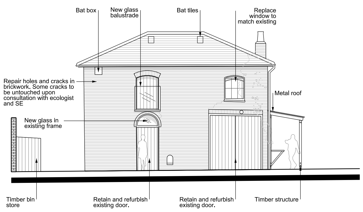
01 0202 Proposed Drawings Stables 1:100@A3 South West Elevation
